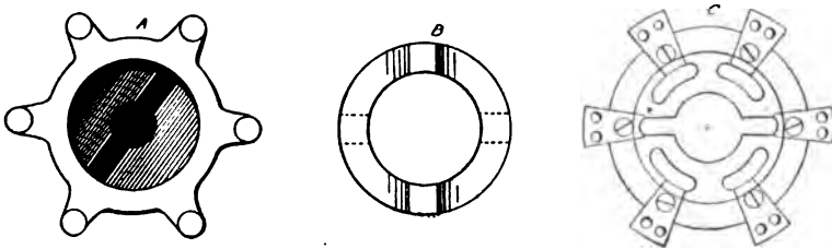
FIG. 130.—Elements of the Compound Hub of the Double Interacting Wheel. A is the outer hub plate, showing interior slot. B is one of the two floating guide plates, carrying keys or splines, arranged on either side, as indicated. C is the central hub plate, also slotted, and arranged for hanging spokes.
